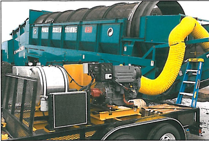
Airlift Separator: AL200D
